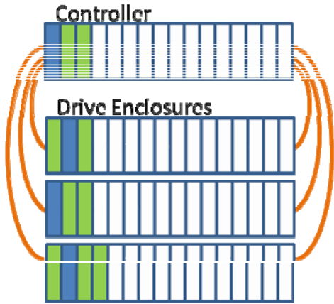
8+1 group striped across even and odd drives of 4 drive enclosures
